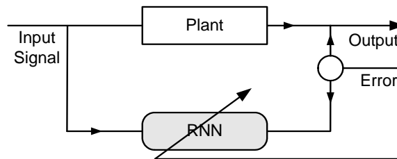
Figure 6.16. System identification using RNN
