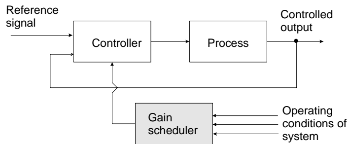
Figure 6.10: Block diagram of the gain scheduling controller
