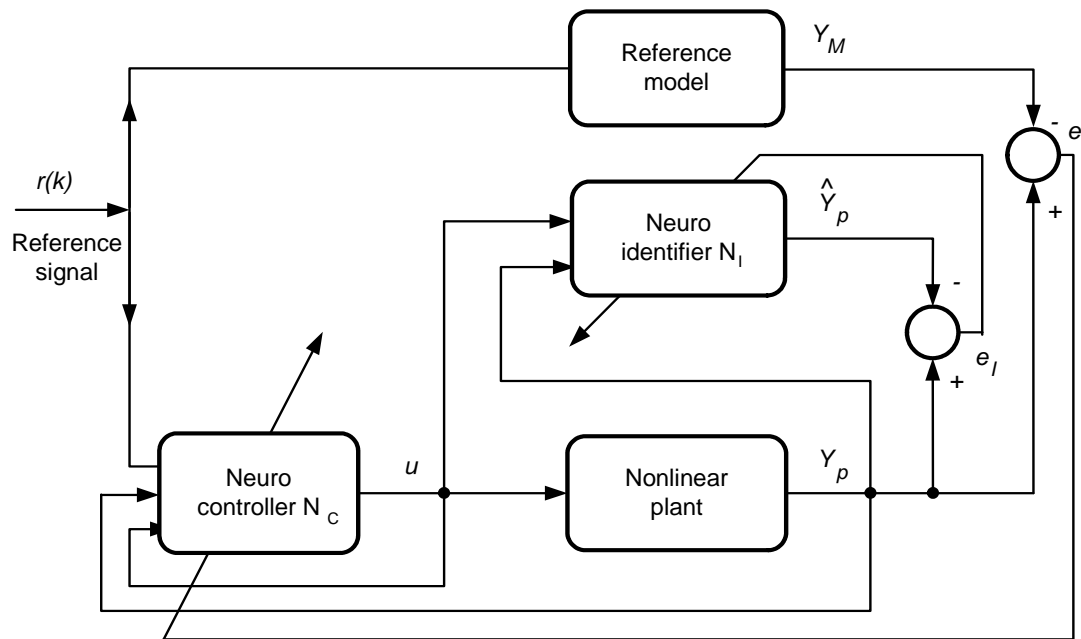
Figure 6.20 Neural network as Neuro Adaptive Controller.
