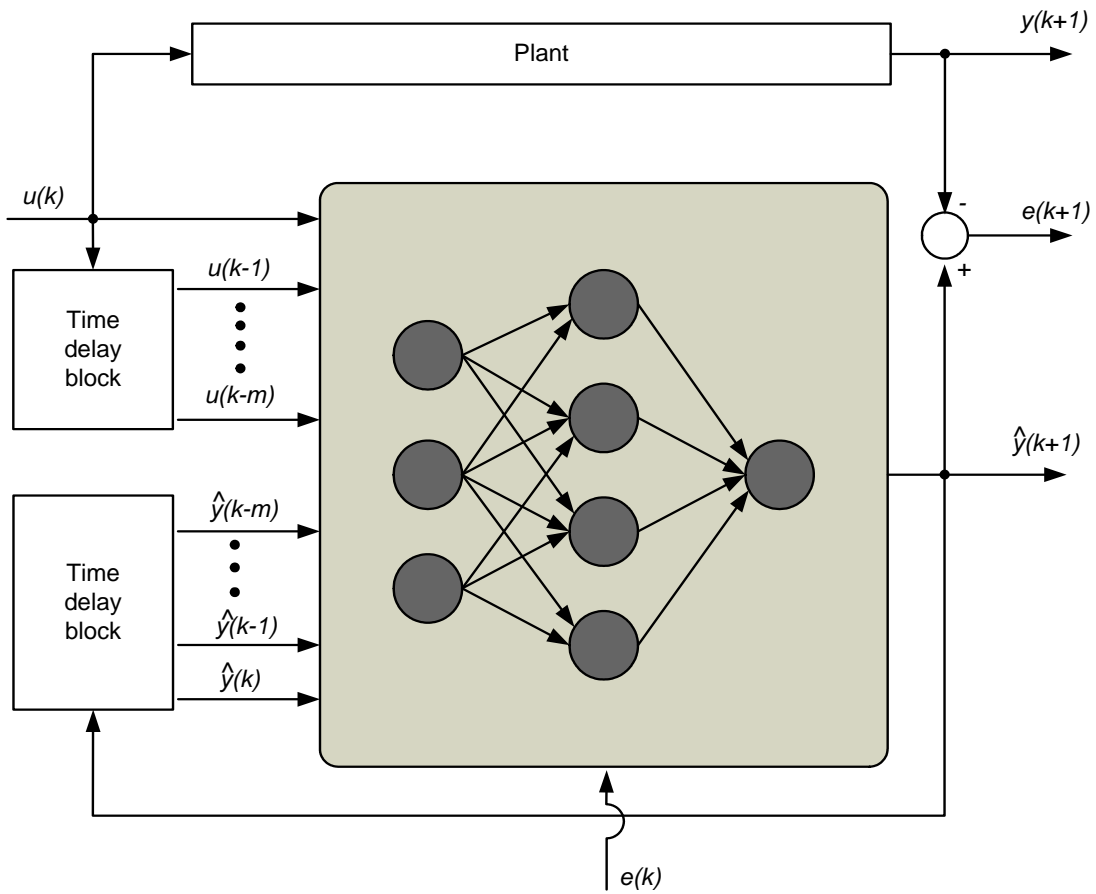
Figure 6.15. Parallel scheme for neural identification
