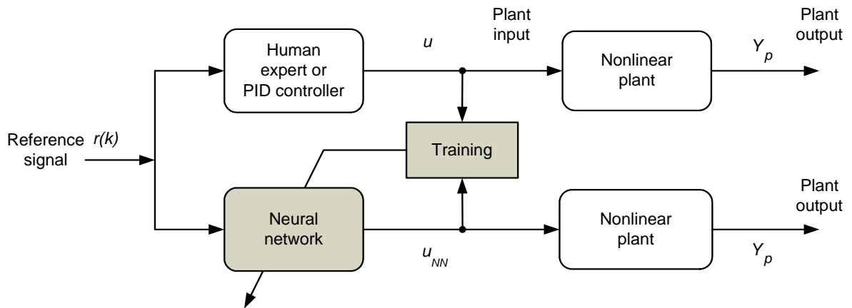
Figure 6.18. Neural network acting as a supervisory controller
