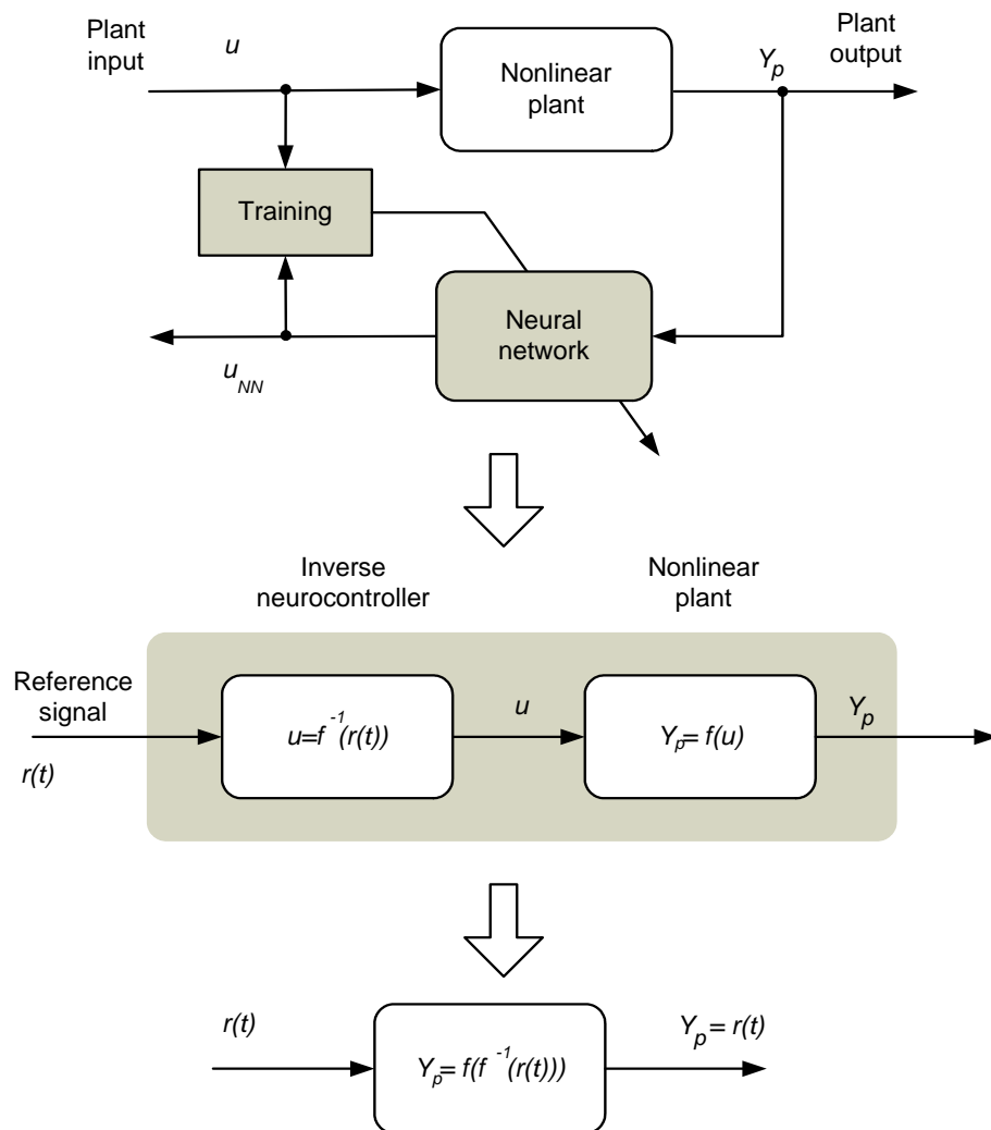
Figure 6.19 Neural network as inverse model based controller
