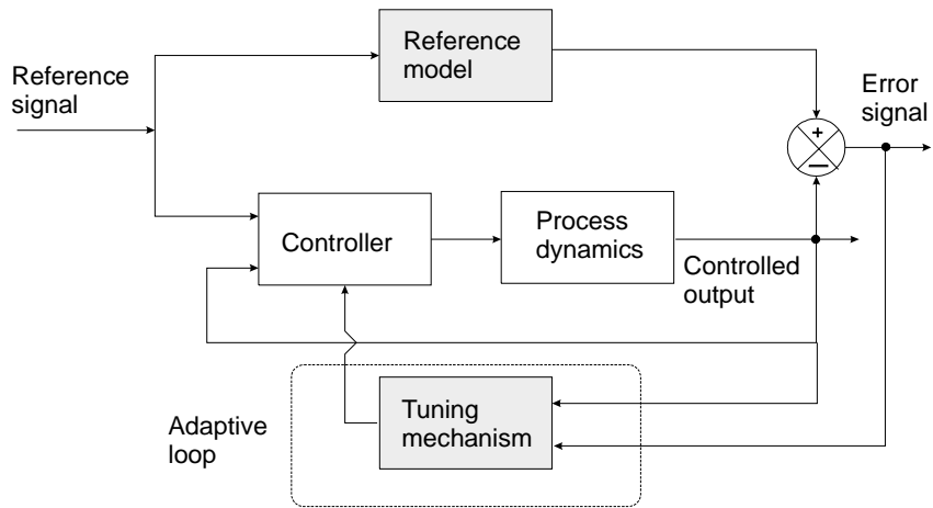
Figure 6.11: Block diagram of a model-referenced adaptive controller
