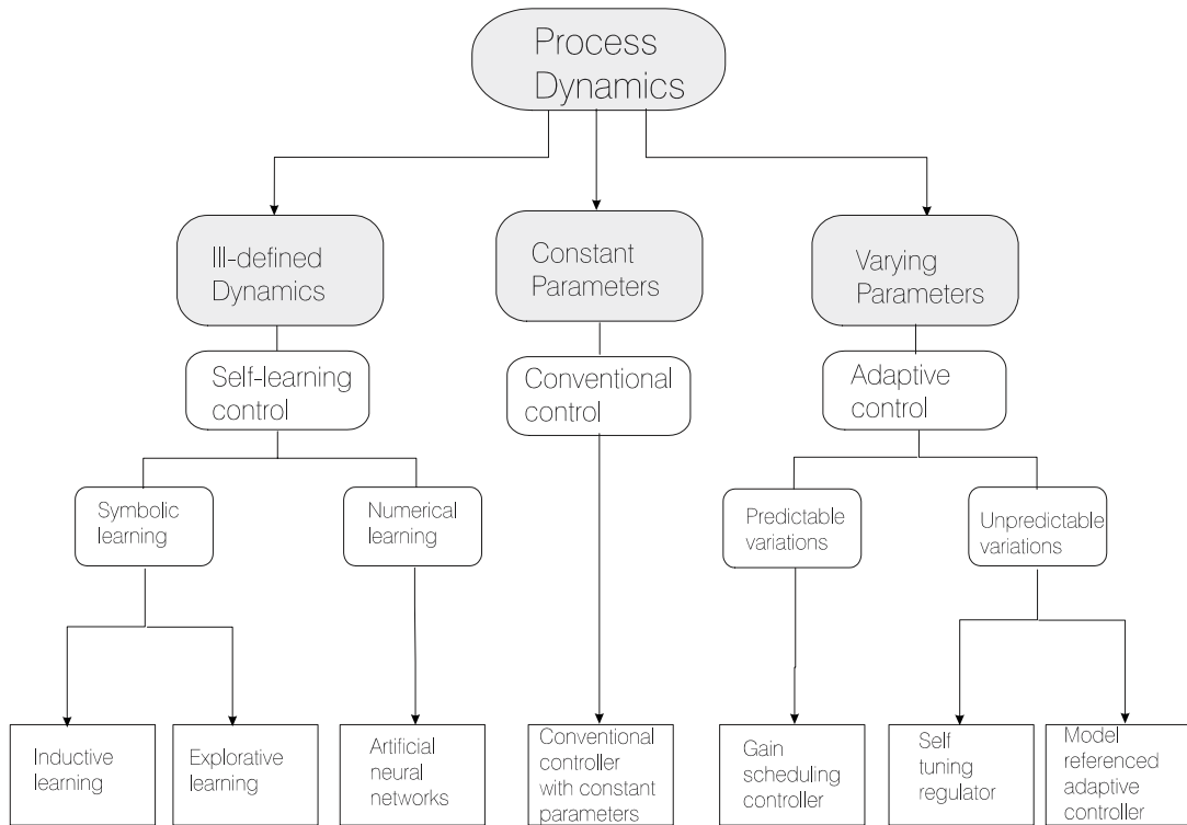
Figure 6.8 Classes of dynamic systems and their appropriate controllers
