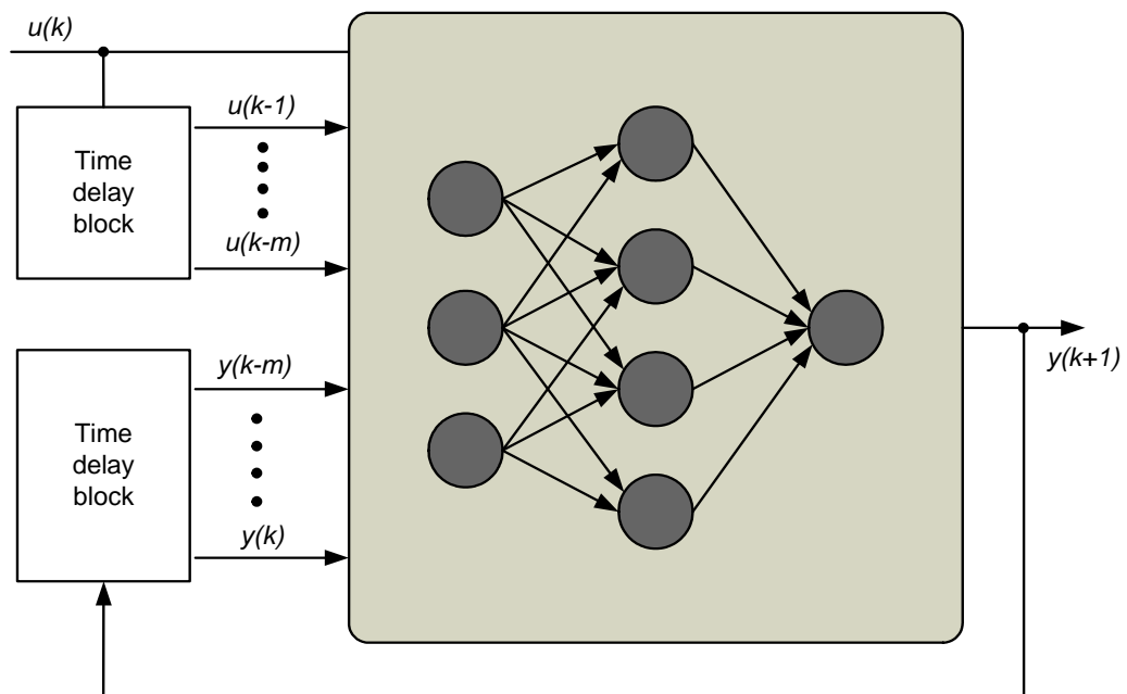
Figure 6.13. Time delayed recurrent neural network
