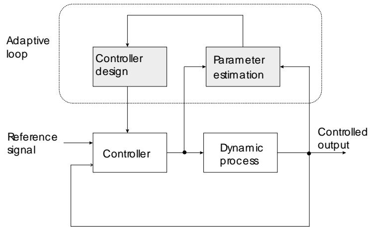
Figure 6.12: Block diagram of the self-tuning regulator
