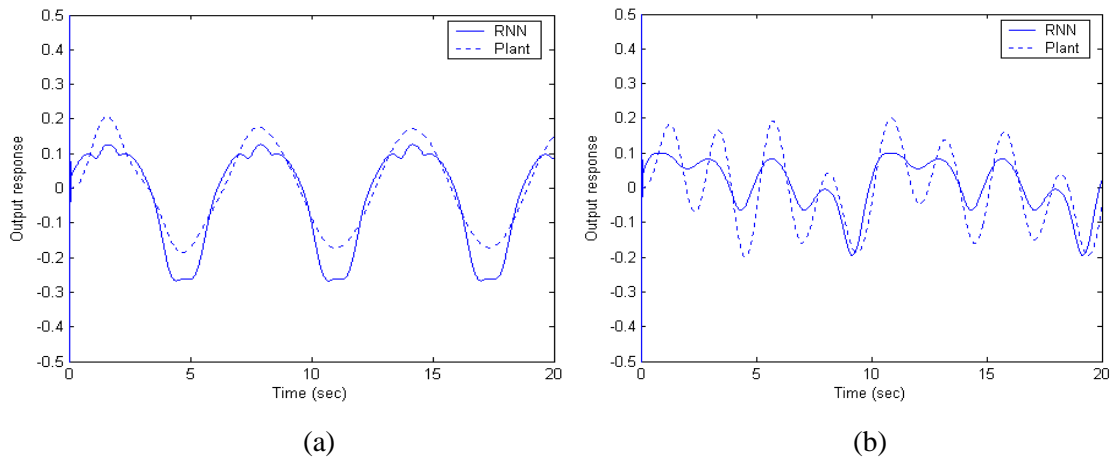
Figure 6.17. (a) Identification results with first set of input, (b) Identification results with second set of input
