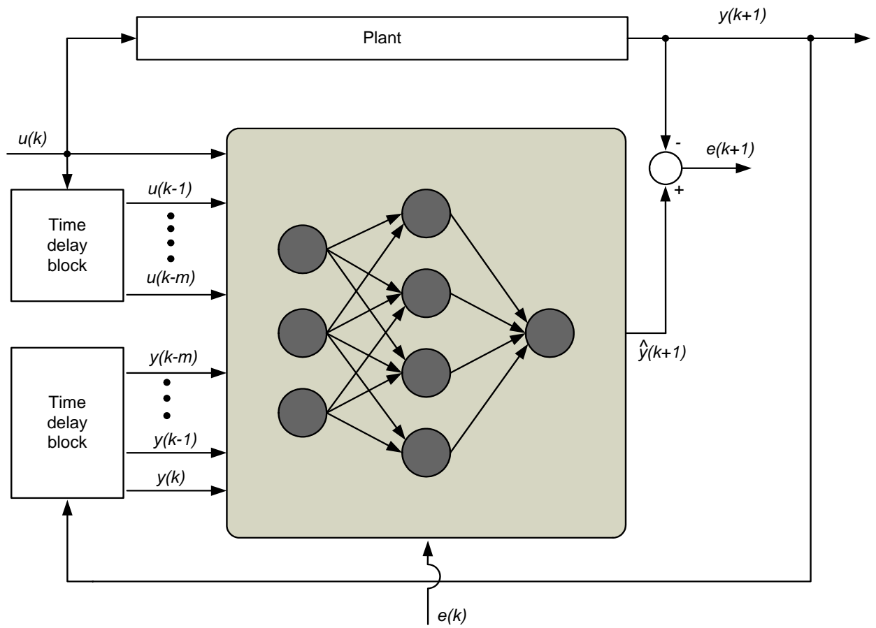
Figure 6.14. Series-parallel scheme for neural identification
